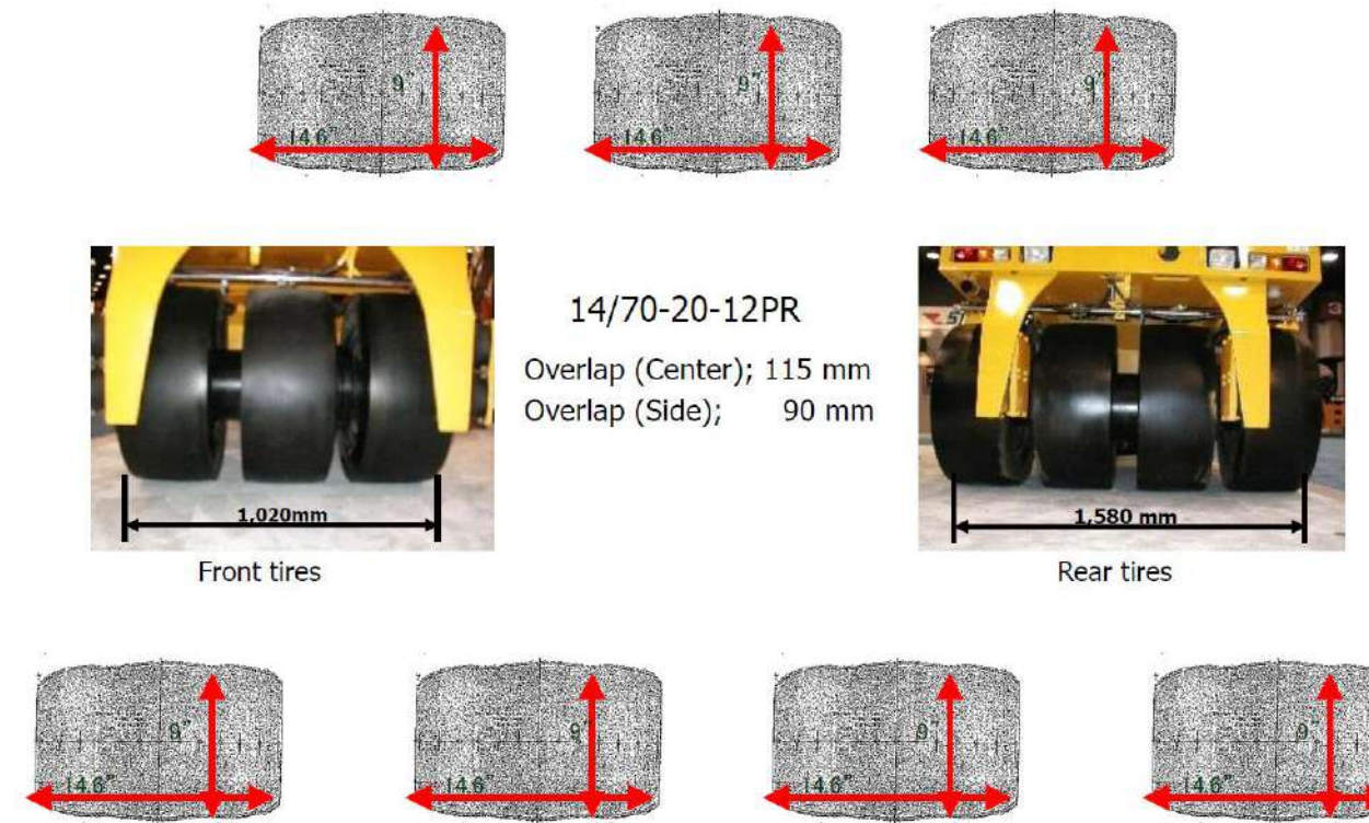
Super Flat Pneumatic Tire
