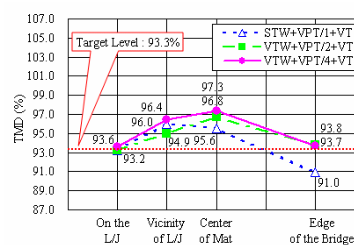
Result of SMA Compaction
