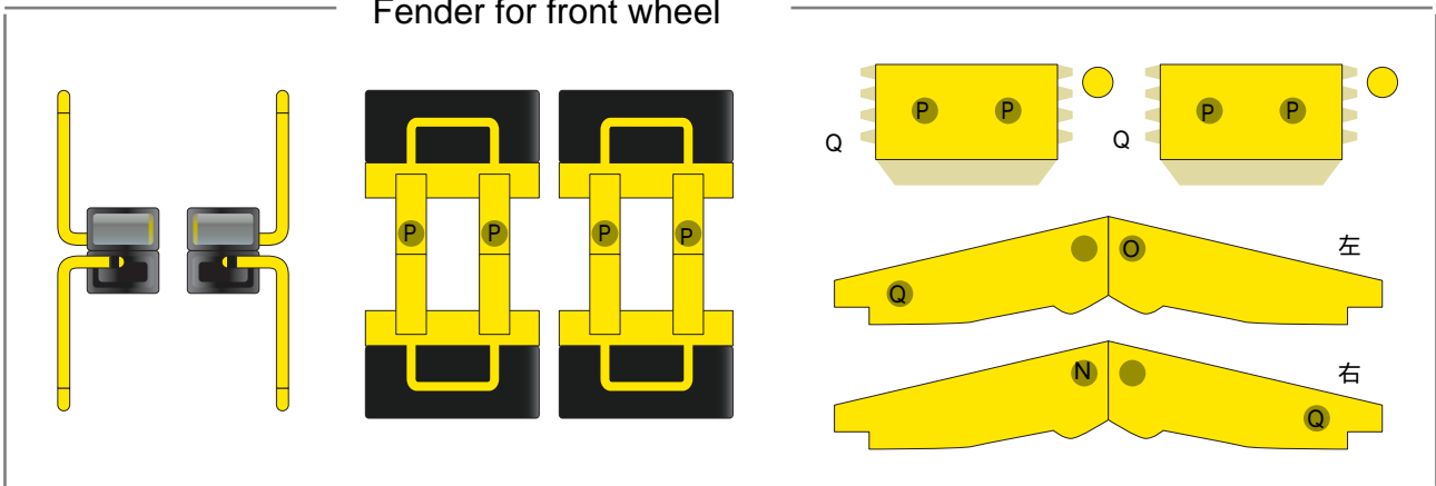
Fender for front wheel
